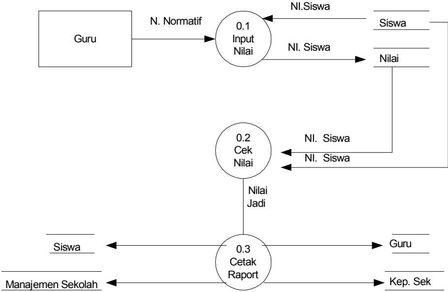
Gambar 4.2 Diagram Zero ( Level 0 )
